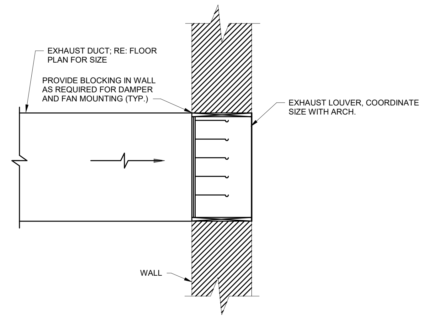
1 EXHAUST SIDEWALL TERMINATION DETAIL NOT TO SCALE
